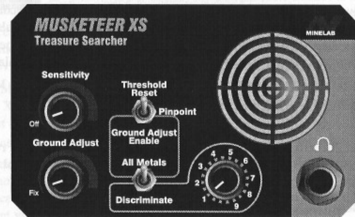
Figure 10 - The Minelab Musketeer XS and XS Pro Control Panel
